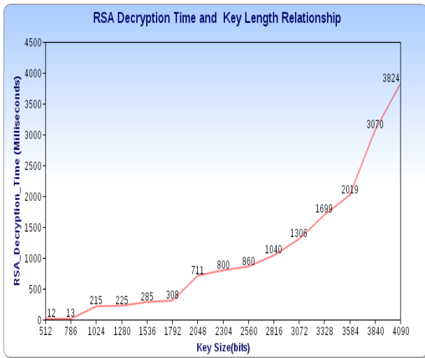
Figure 2: Graph between RSA Decryption Time and Key Length
