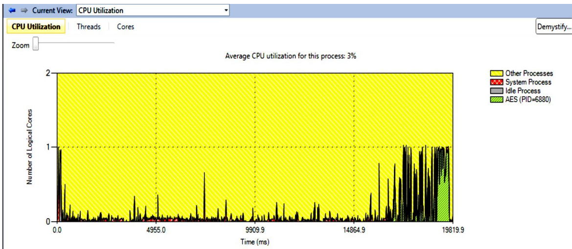
Figure 7: AES CPU Utilization
