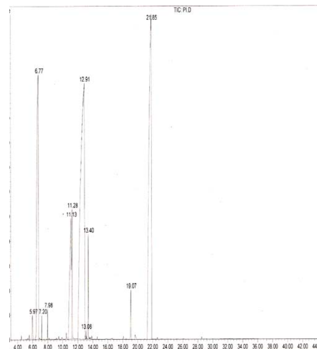
Fig. 1: GC-MS chromatogram of the essential oil of Anethum graveolens L.
